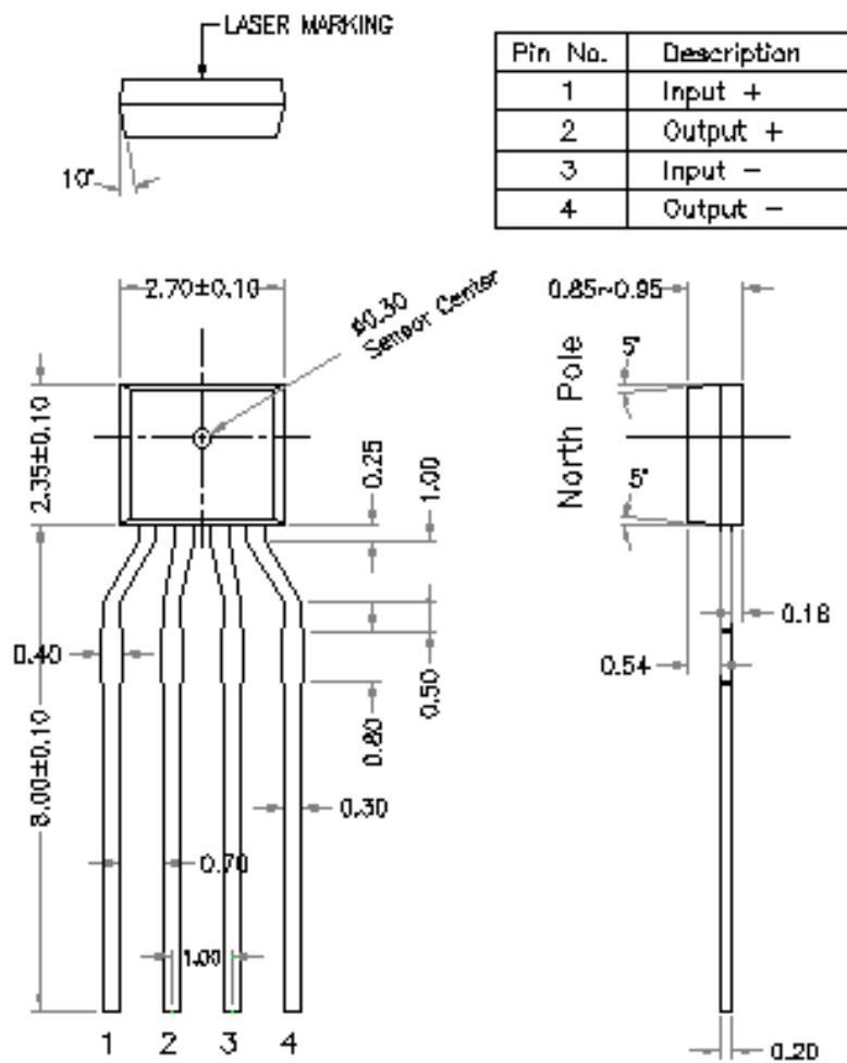
[Package Dimensions]
